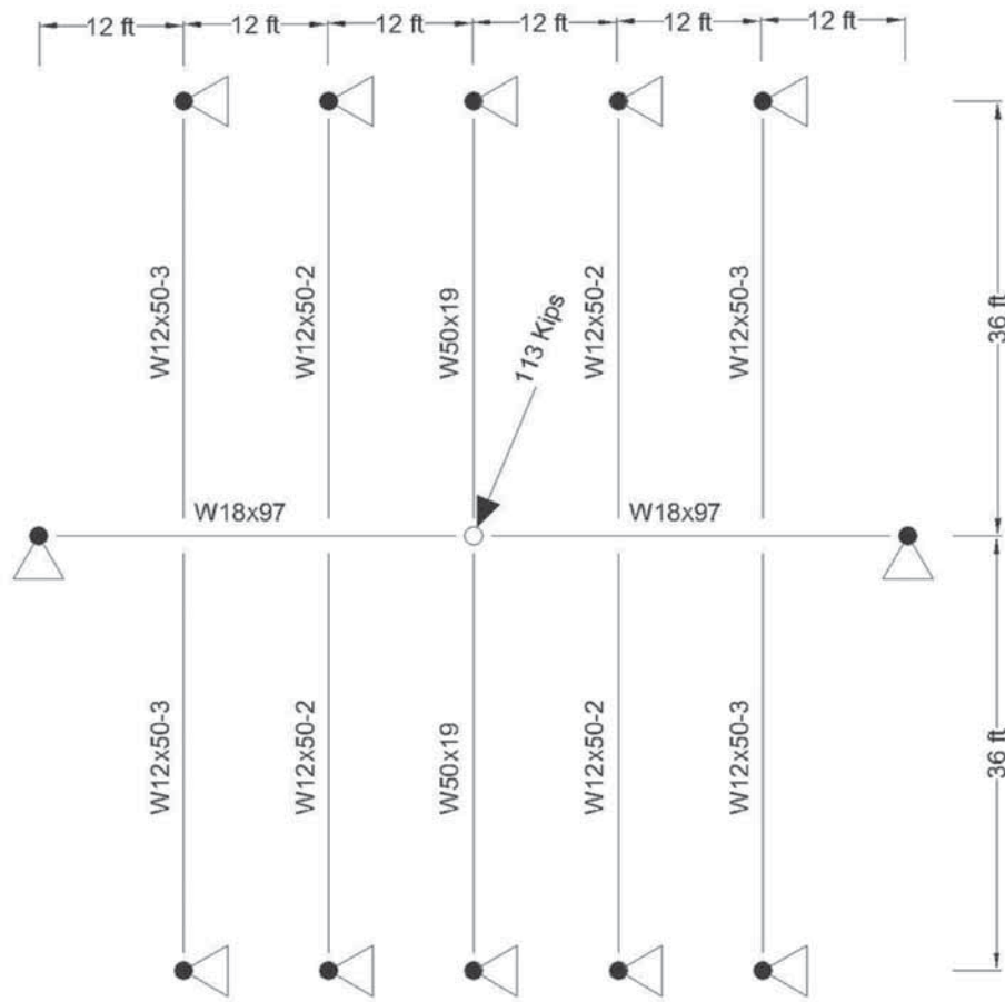
Fig. 8-14. Model B.
