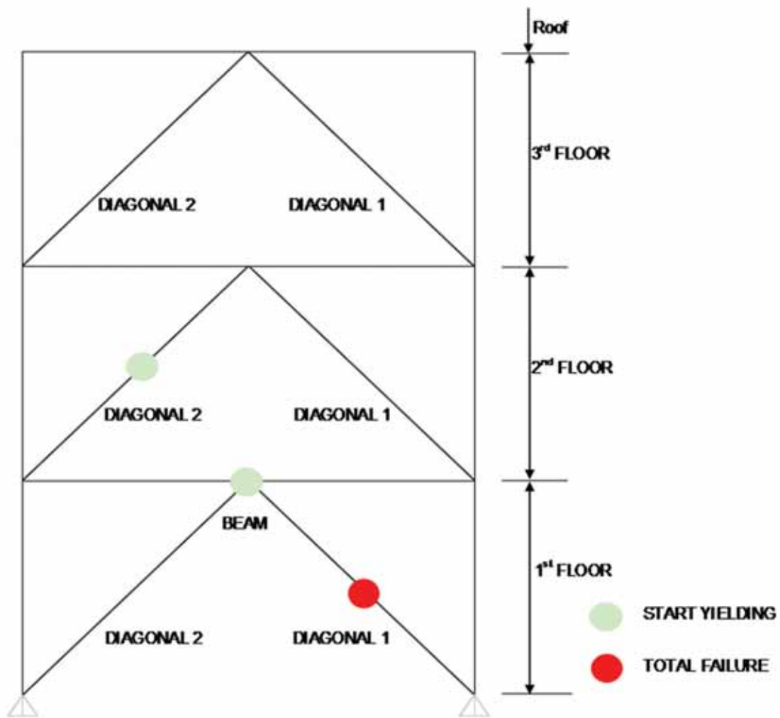
Fig. 5-21. Element response.
