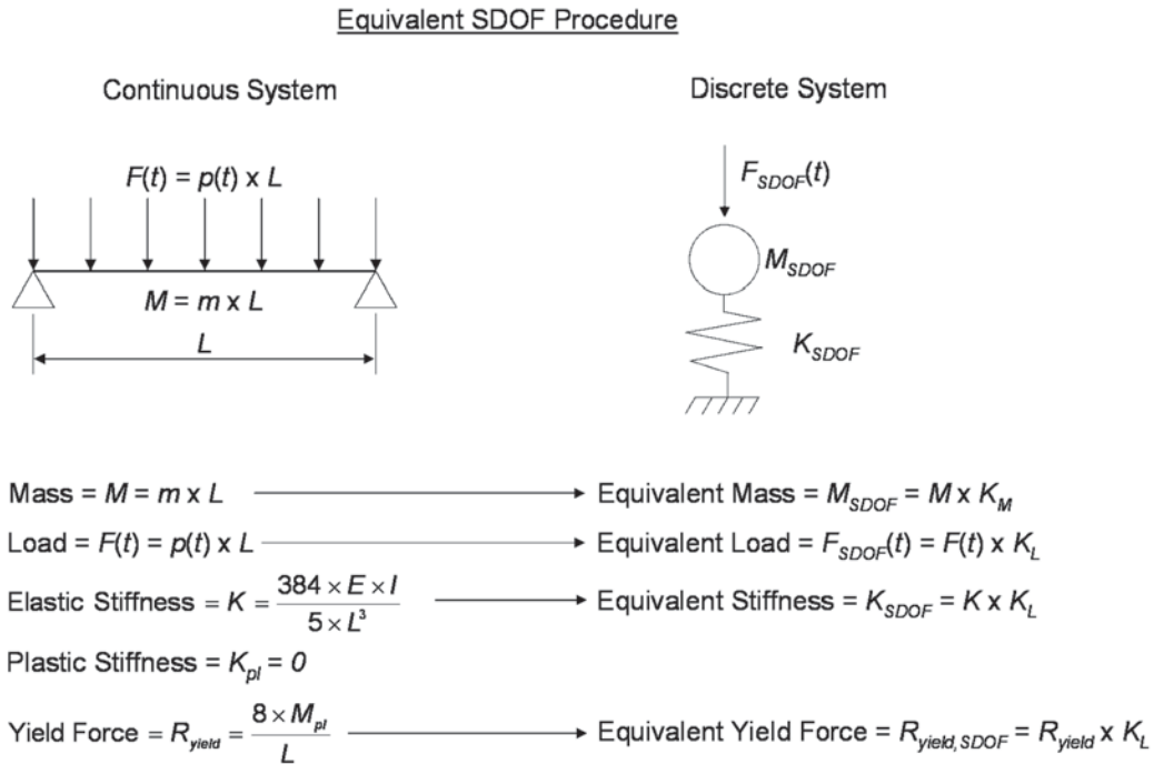
Fig. 6-10. MDOF-to-SDOF simplification.
